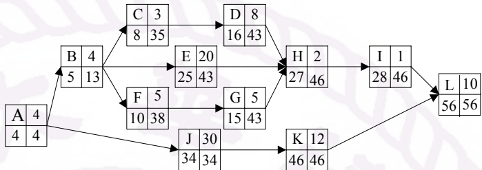
Fig.2 Example timed workflow graph
